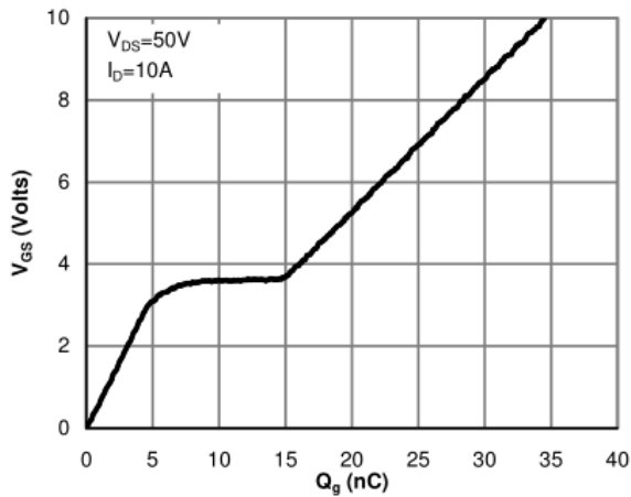
Figure 2: Gate Charge Characteristics
